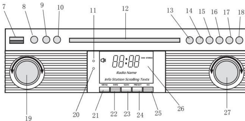
FRONT PANEL
